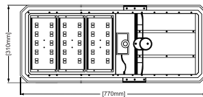
Dimension ( mm )
