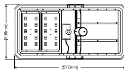
Dimension ( mm )
