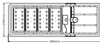
Dimension ( mm )
